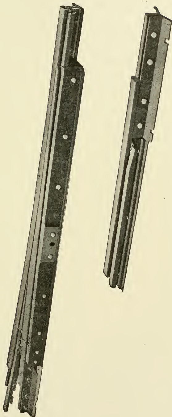
Fig. 235. Typical Steel Track Form. "Switch" in Two Parts
